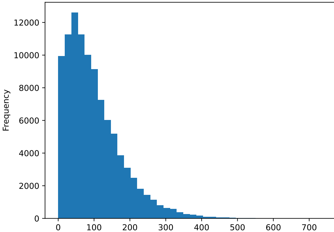
post-selection, 1e+01
