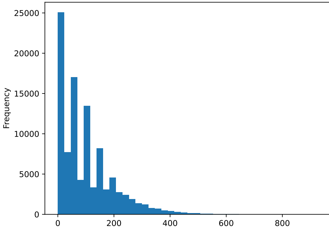
post-selection, 2
