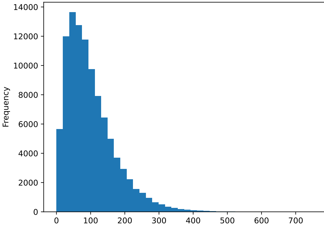
pre-selection counts/variant
